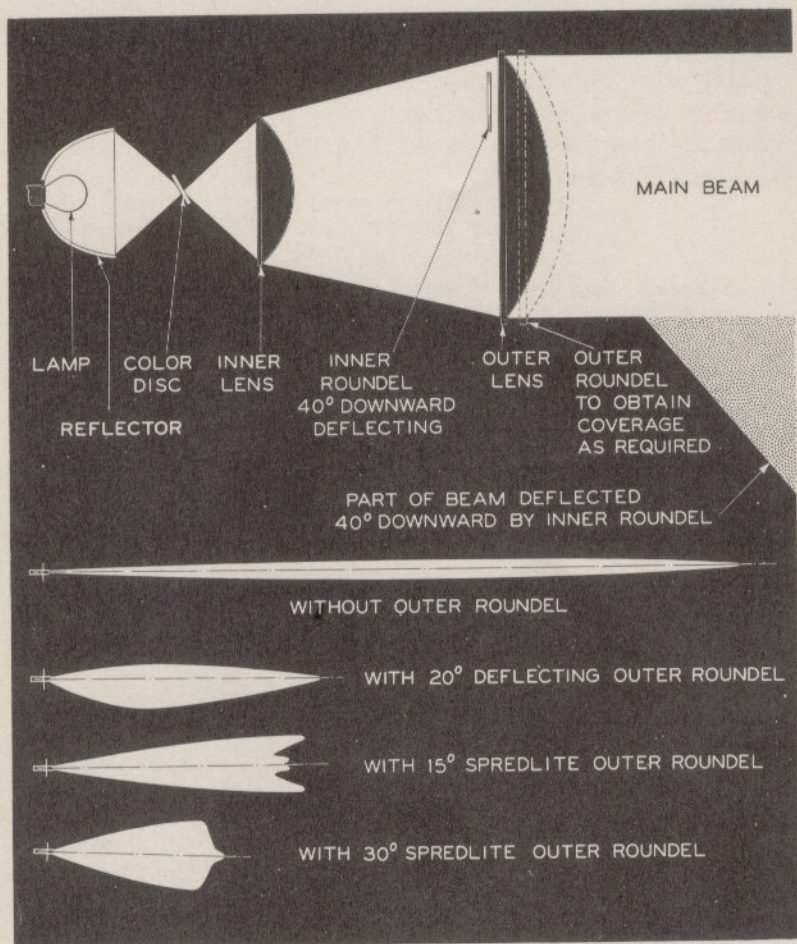
Figure 14. Compound-lens system showing beam coverages with different lens combinations. Lens system shown viewed from side of signal; beam coverages shown looking down on track.
