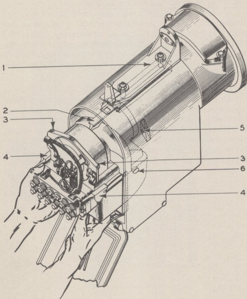
Figure 4. Inserting the signal operating mechanism into the housing.
