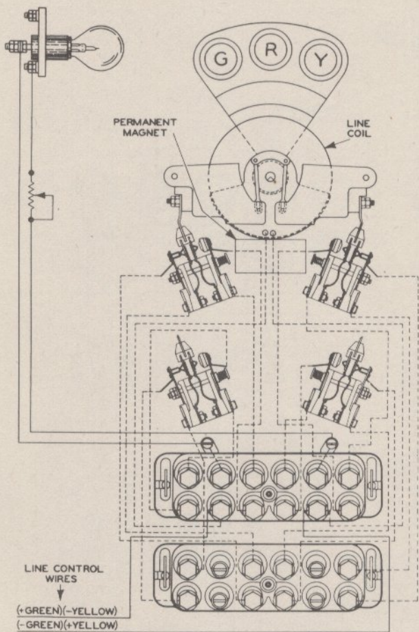
Figure 7. Simplified diagram of Type SA d-c. signal operating mechanism with 8 independent contacts and 2 plug couplers. Dotted lines indicate internal wiring. Solid lines indicate external wiring.
