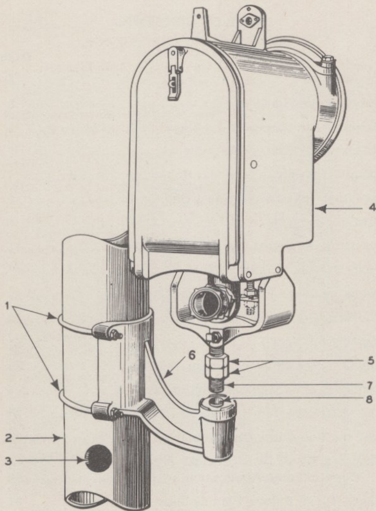
Figure 1. Mounting the Type SA signal housing on the side of the mast.
