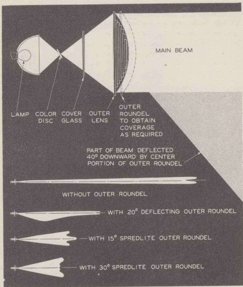
Figure 15. Stepped-lens system showing beam coverages with different lens combinations. Lens system shown viewed from side of signal; beam coverages shown looking down on track.
