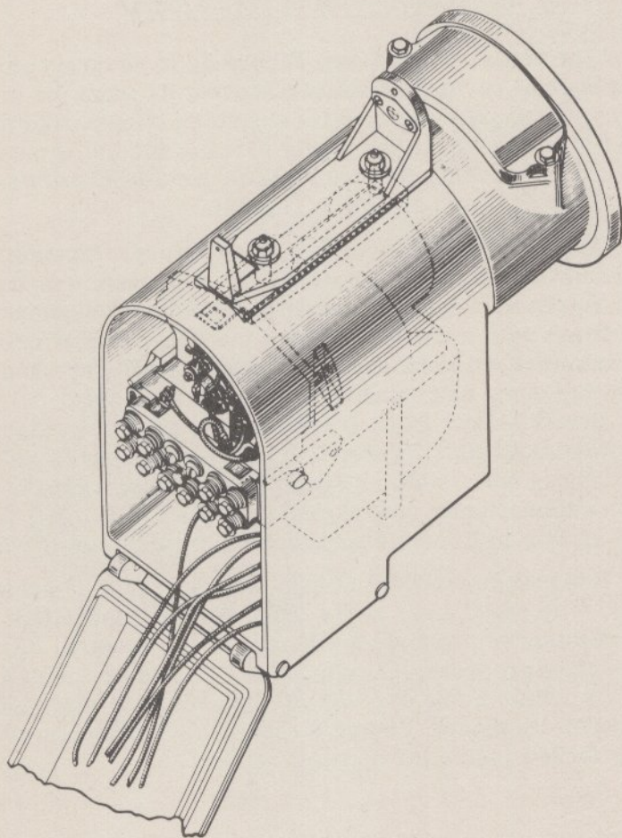
Figure 5. Signal operating mechanism properly positioned and locked in the signal housing.
