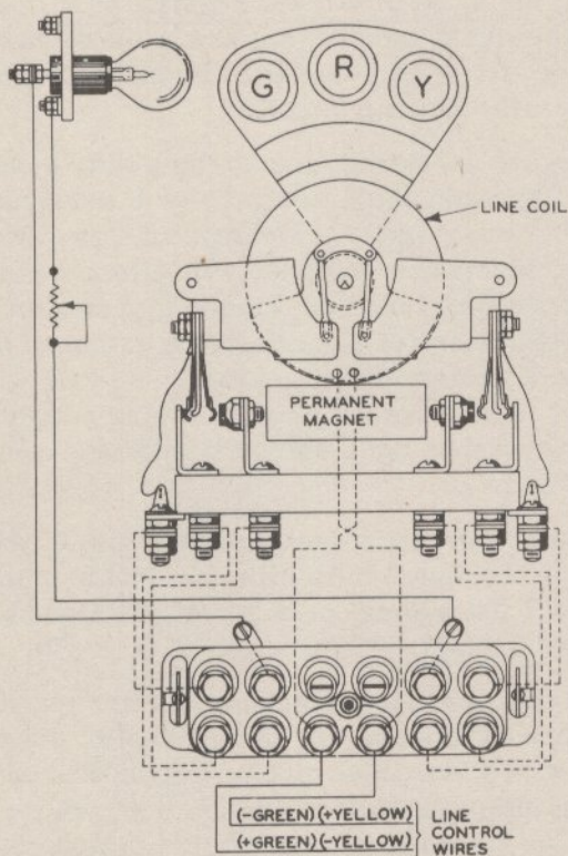
Figure 6. Simplified diagram of Type SA d-c. signal operating mechanism with two dependent front and back contacts. Dotted lines indicate internal wiring. Solid lines indicate external wiring. Plug coupler is shown. Wiring is same on models equipped with terminal blocks (except lamp and resistor, which are connected as shown in Figure 8).
