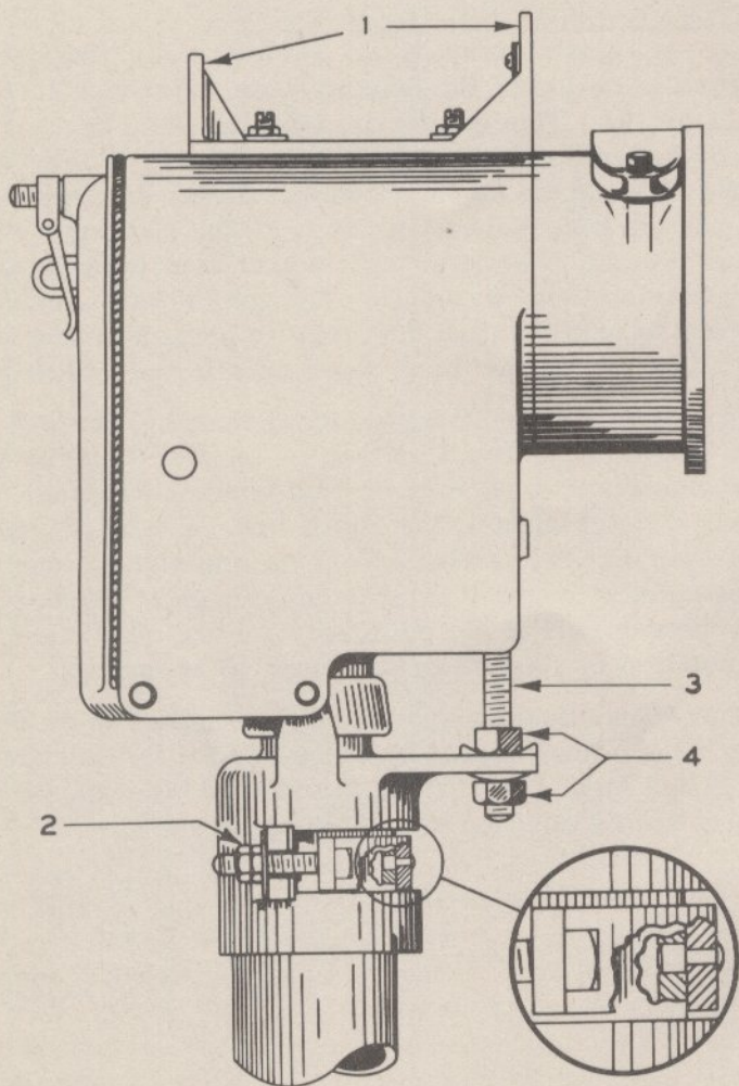
Figure 12. Sighting the Type SA top-of-mast signal.
