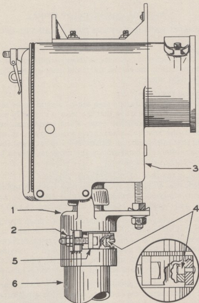
Figure 2. Mounting the Type SA signal housing on the top of the mast.
