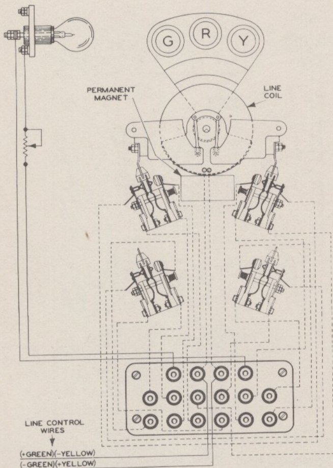
Figure 8. Simplified diagram of Type SA d-c. signal operating mechanism with 8 independent contacts and 3-row terminal block. Dotted lines indicate internal wiring. Solid lines indicate external wiring.
